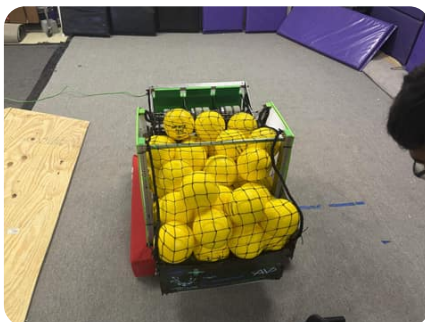
55 ball capacity big dumper archetype front view
